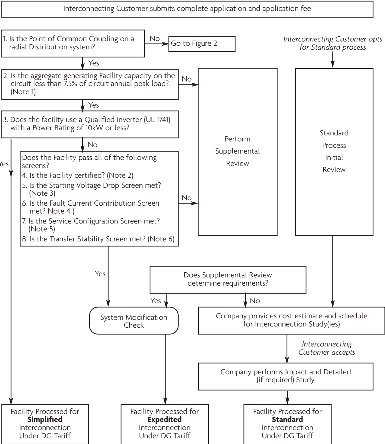
Figure 1 SCHEMATIC OF MASSACHUSETTS DG INTERCONNECTION PROCESS
